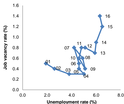
Graph 1.6: Beveridge curve
