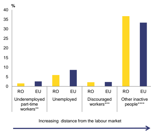
Graph 3.3.2: Activation potential*
