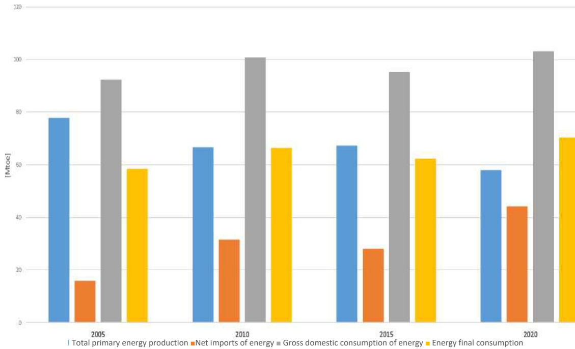
Figure 2.20. National energy balance 2005-2020
